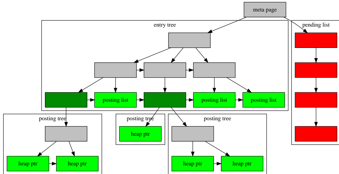
Figure 64.1. GIN Internals
